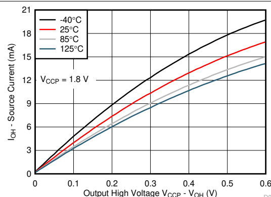
Figure 6-12. I/O Source Current vs Output High Voltage ( V_{CCP} = 1.8\text{ V} )
