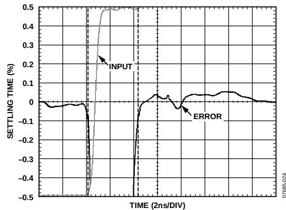
Figure 31. Settling Time
