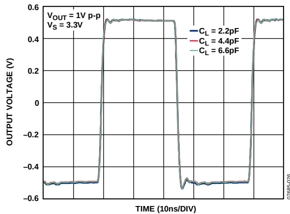
Figure 30. Large Signal Transient Response vs. Capacitive Load
