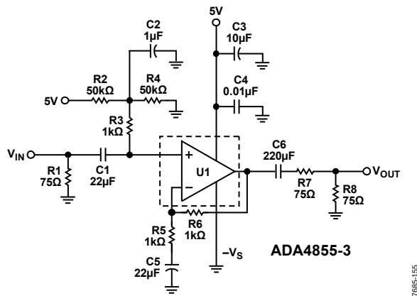
Figure 54. AC-Coupled, Single-Supply Video Driver Schematic
