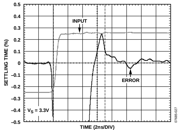
Figure 34. Settling Time
