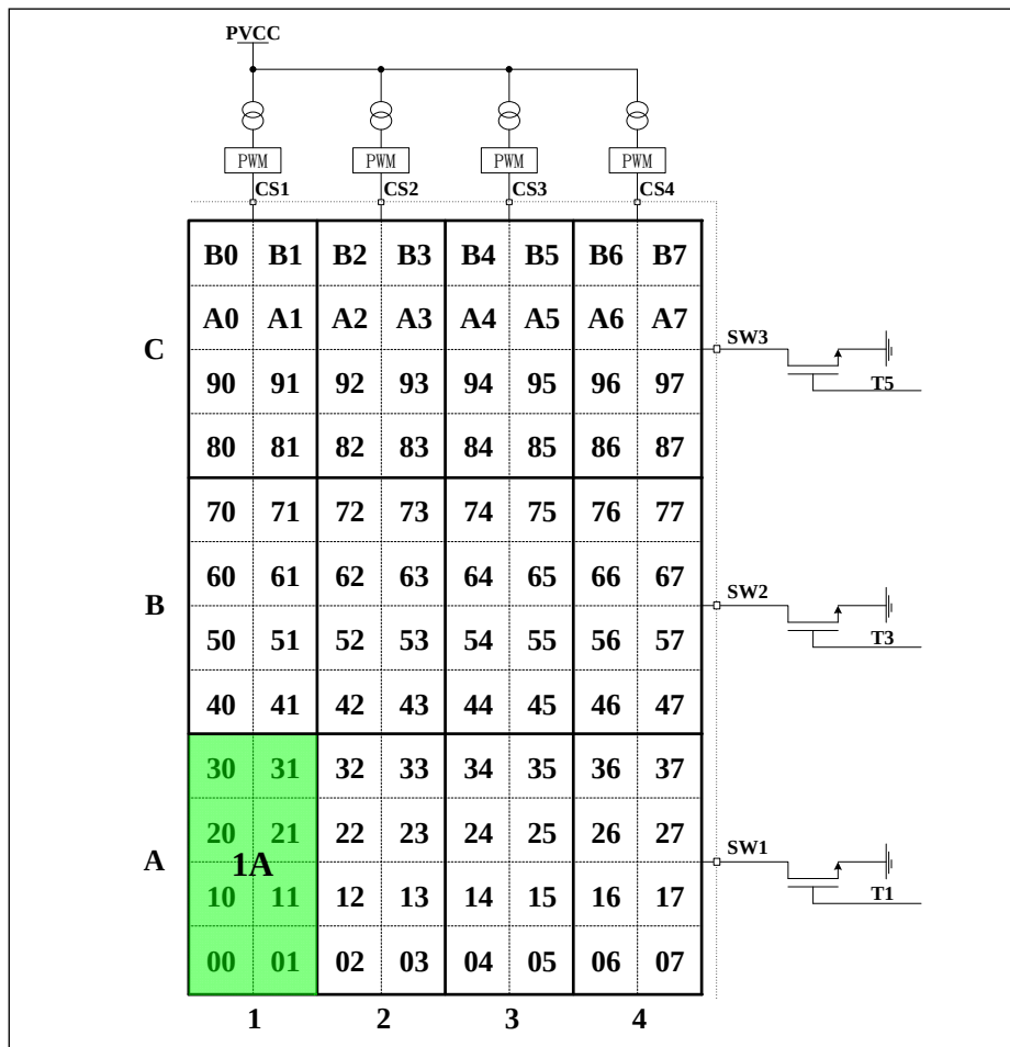
Figure 12 PWM Register
