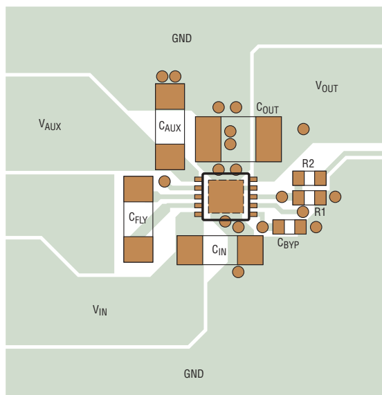
BOOST LAYOUT
