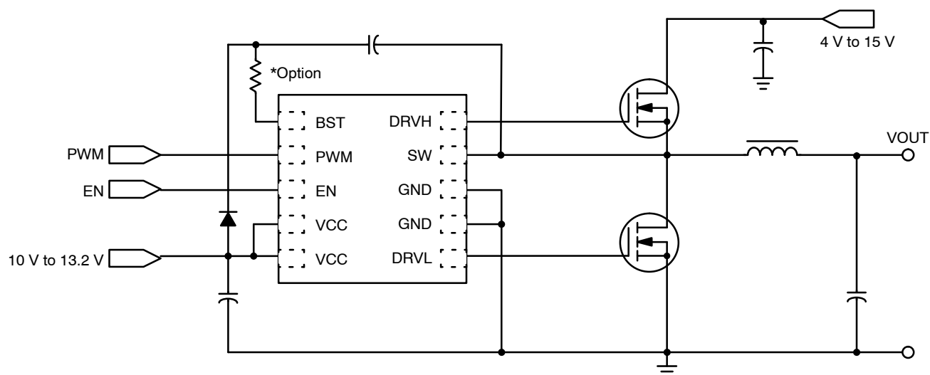
Figure 2. Typical Application
