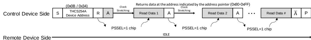
Figure 17 2-wire serial controller register access protocol (2)
