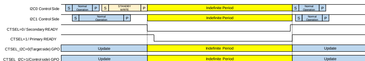
Figure 30 Standby => Normal (CTSEL_I2C=0/Secondary , CTSEL_I2C=1/Primary)
