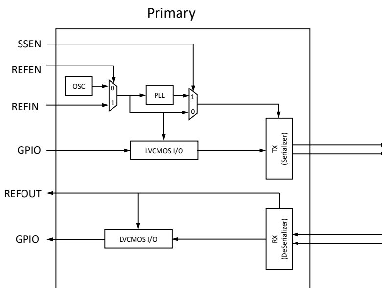
Figure 2 Clock Tree diagram of Primary chip
