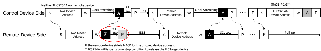
Figure 19 2-wire serial remote device access protocol (1)
