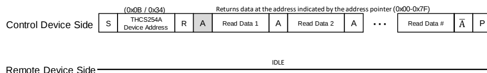
Figure 14 2-wire serial target register access protocol (2)
