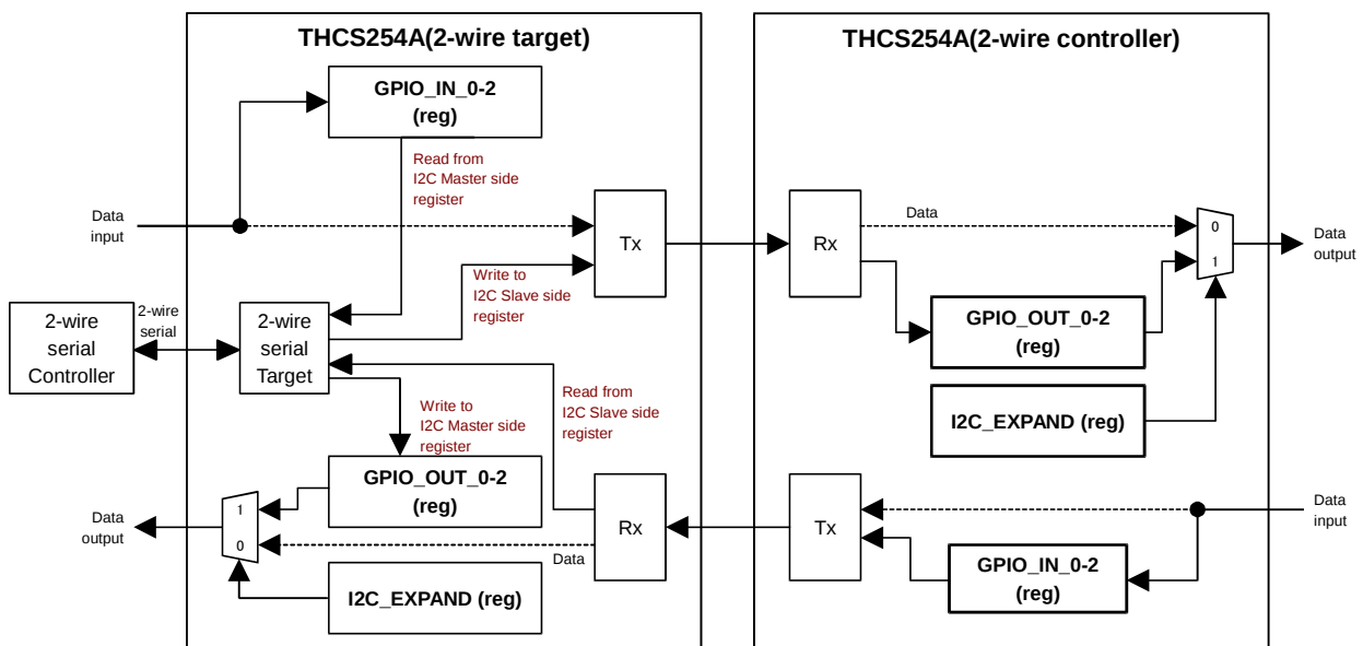
Figure 22 2-wire serial expander function
