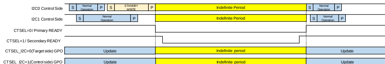
Figure 27 Normal => Standby (CTSEL_I2C=0/Primary , CTSEL_I2C=1/Secondary)
