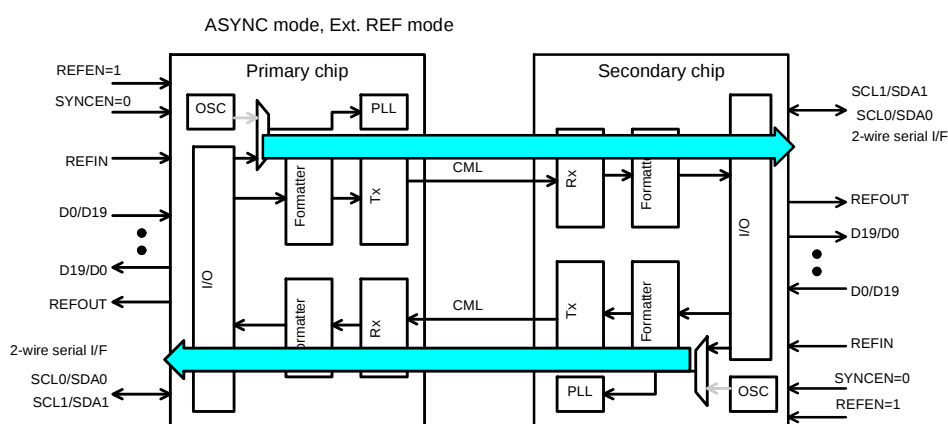
Figure 4 ASYNC_MODE / Ext.REF_MODE Block diagram
