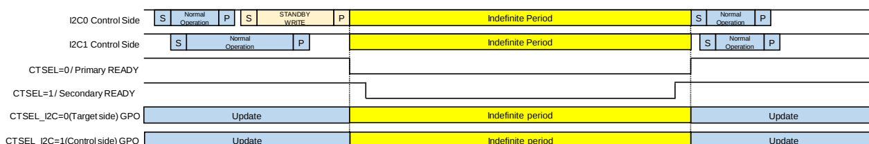
Figure 29 Standby => Normal (CTSEL_I2C=0/Primary , CTSEL_I2C=1/Secondary)
