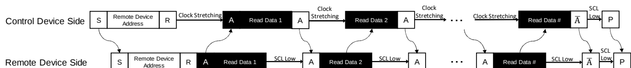
Figure 20 2-wire serial remote device access protocol (2)
