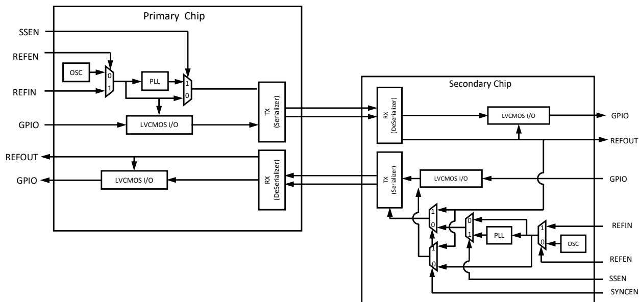
Figure 25 Spread Spectrum Configuration
