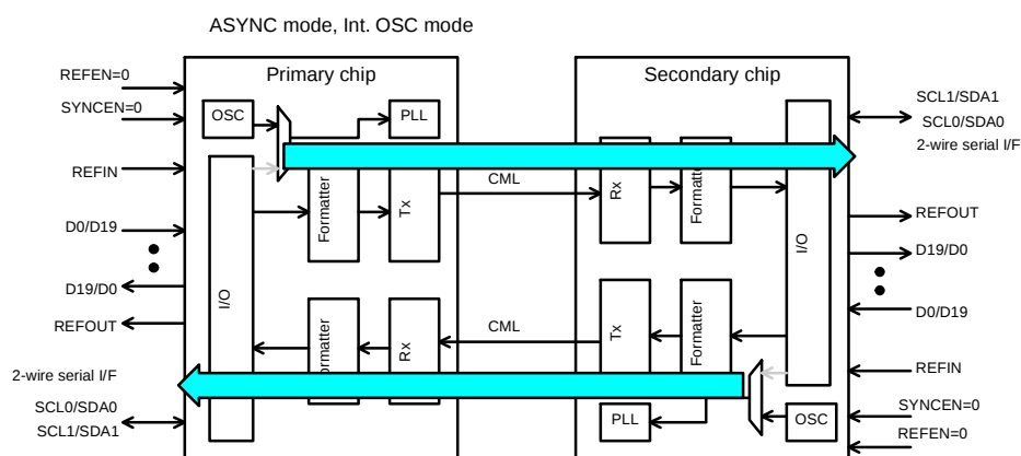
Figure 5 ASYNC_MODE / Int. OSC_MODE Block diagram
