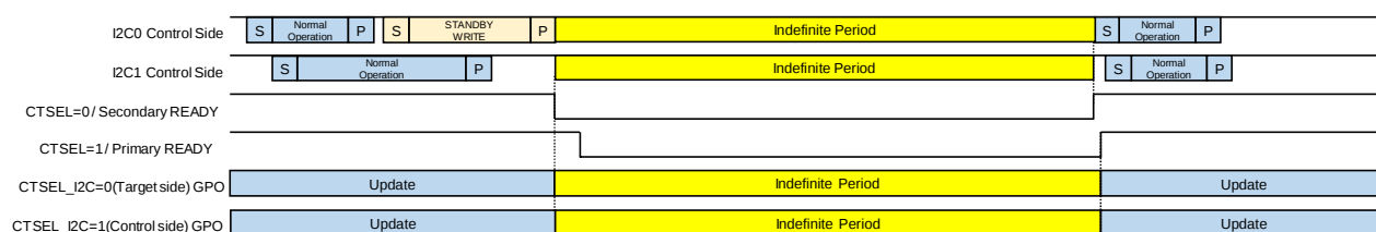
Figure 28 Normal => Standby (CTSEL_I2C=0/Secondary , CTSEL_I2C=1/Primary)
