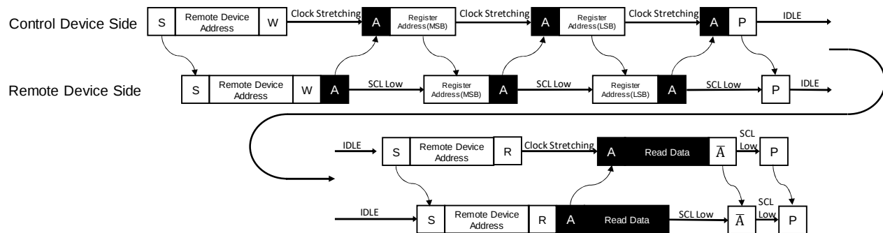
Figure 21 2-wire serial remote device access protocol (3)
