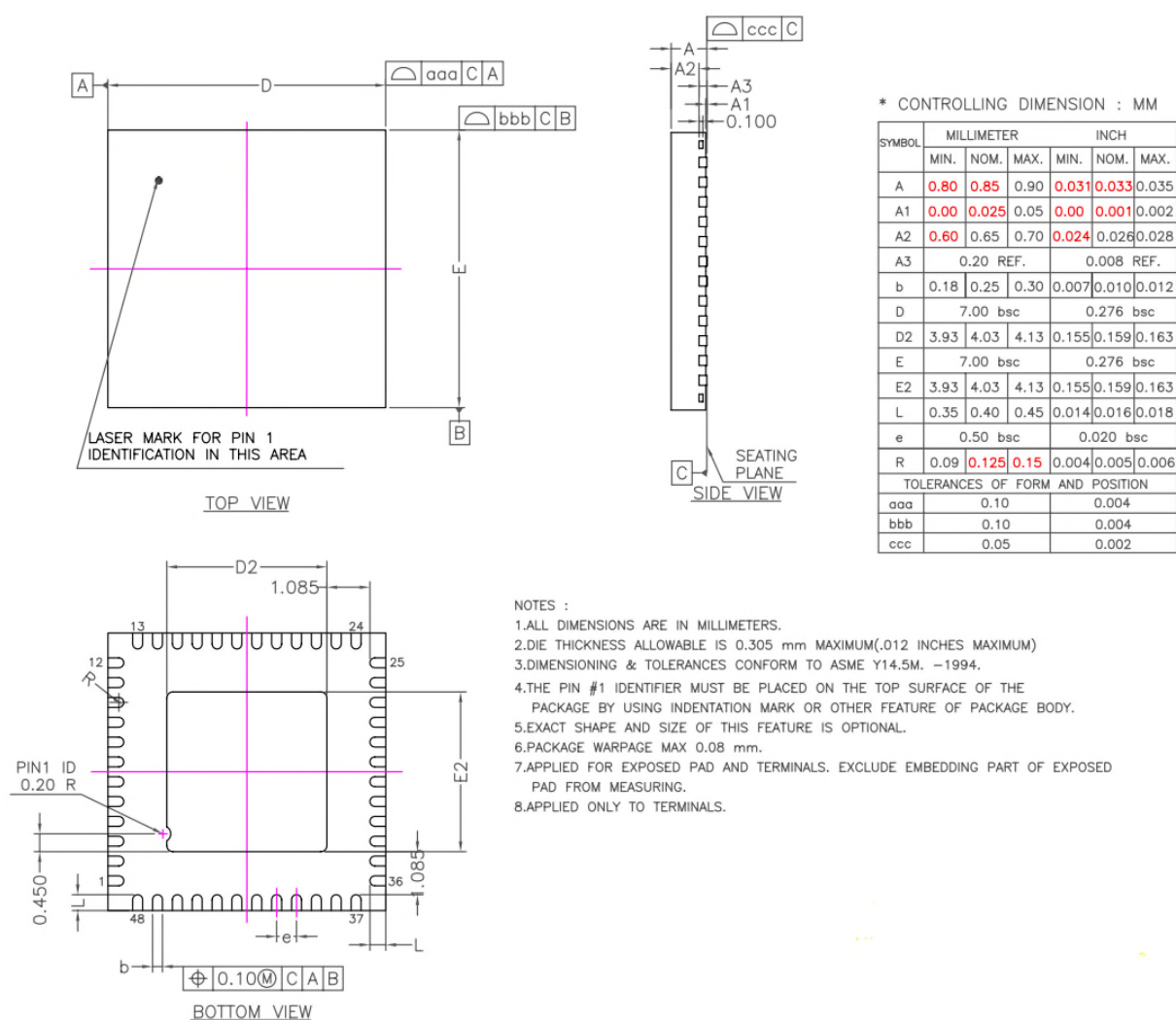
Figure 31 48-pin QFN package physical dimension
