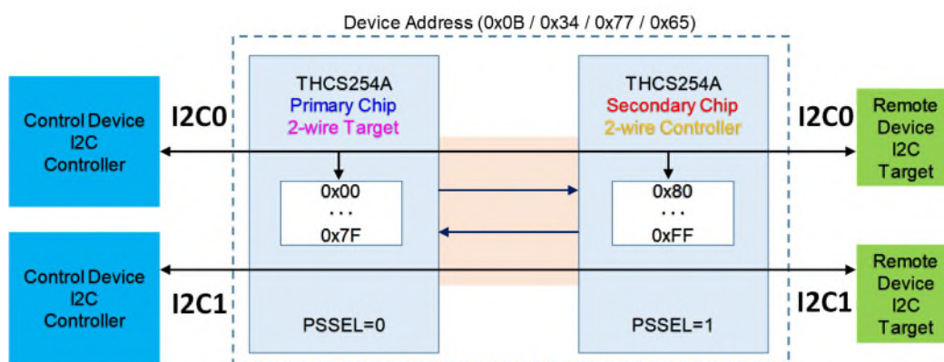
Figure 9 2-wire serial interface accessible range
