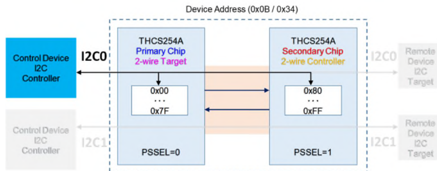
Figure 15 2-wire serial controller register access
