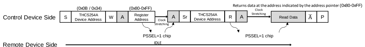
Figure 16 2-wire serial controller register access protocol (1)
