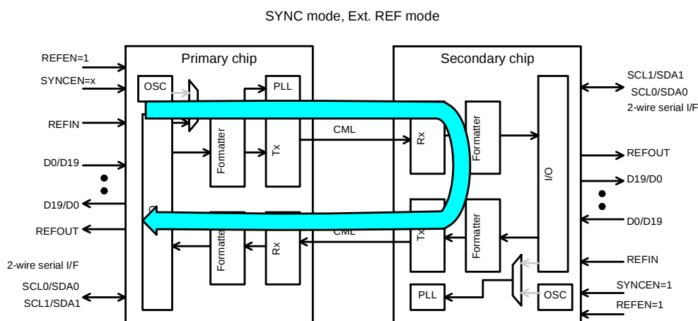
Figure 7 SYNC_MODE / Ext.REF_MODE Block diagram
