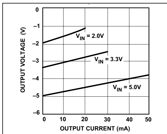
FIGURE 2-10: Output Voltage vs. Output Current.
