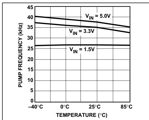
FIGURE 2-9: TCM829 – Pump Frequency vs. Temperature.
