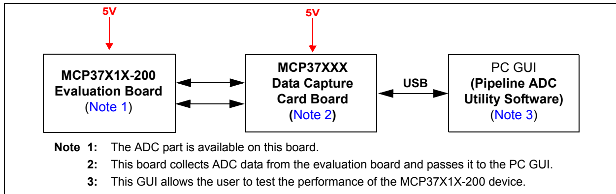
FIGURE 1-1: Evaluation Kit System Setup.
