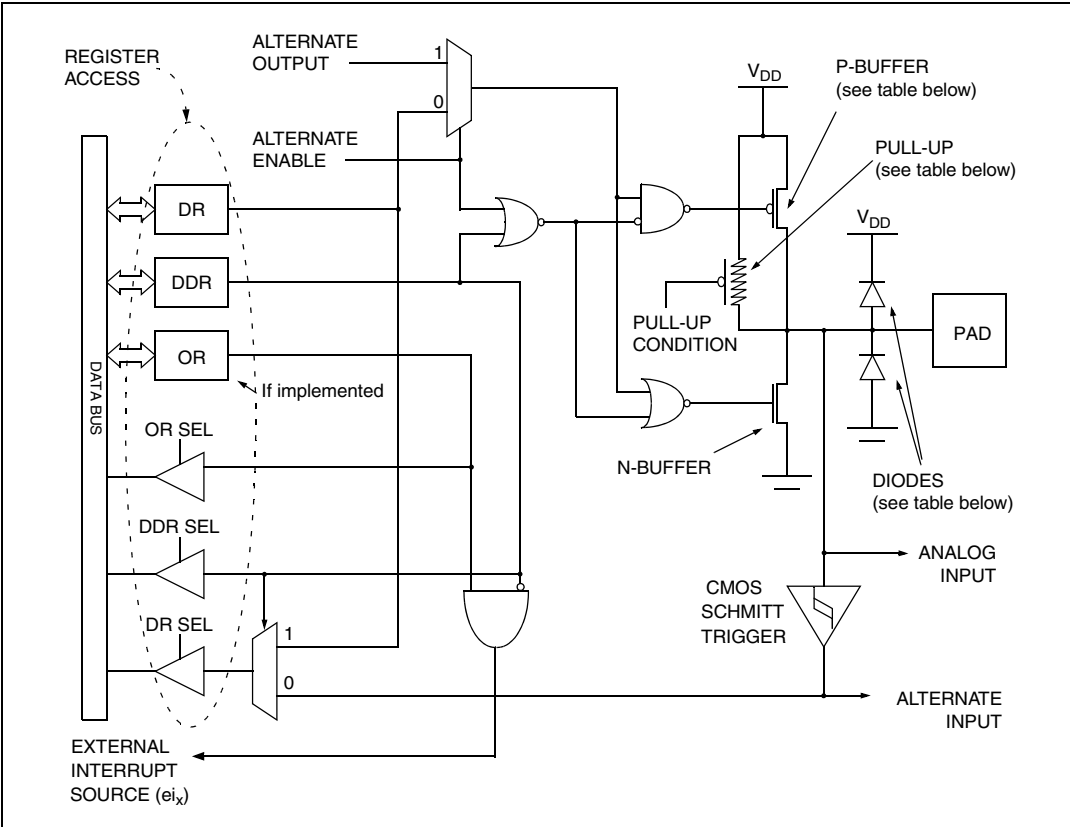
Figure 25. I/O port general block diagram
