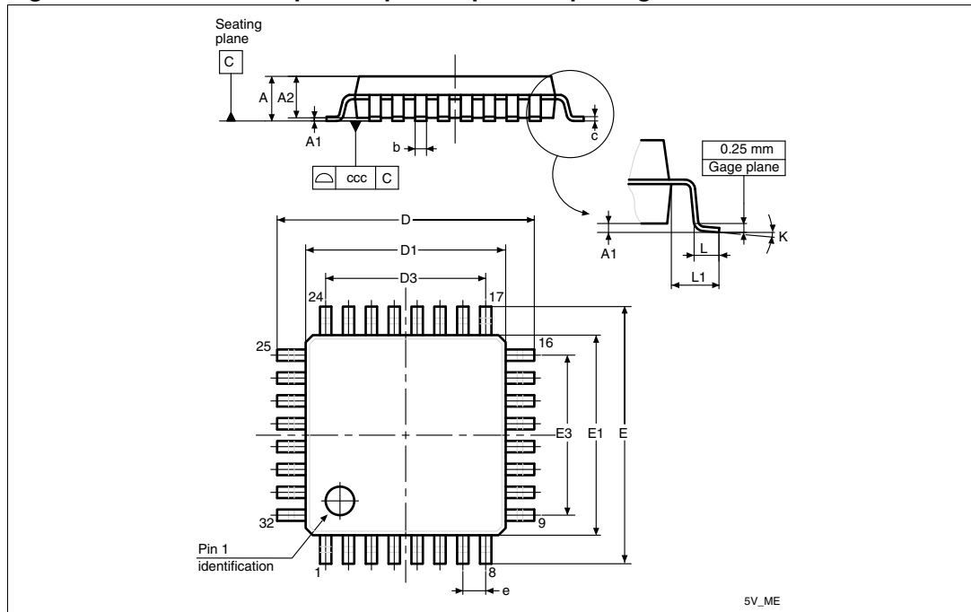
Figure 91. LQFP32 – 32-pin low-profile quad flat package outline
