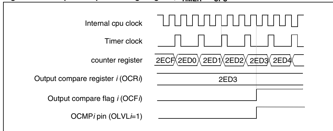
Figure 39. Output compare timing diagram, f_{\text{TIMER}} = f_{\text{CPU}}/4
