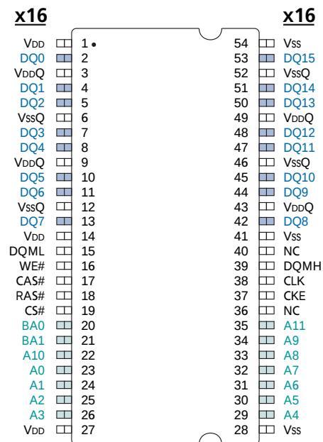
Figure 5: 54-Pin TSOP Pin Assignments (Top View)
