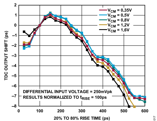
Figure 17. TDC Output Shift vs. Incoming BSYNC Time Rise for Various Common-Mode Voltages
