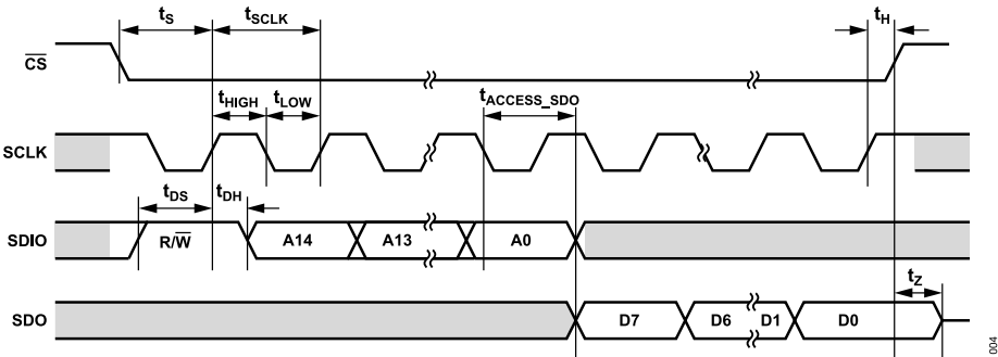
Figure 4. 4-Wire Read Timing Diagram
