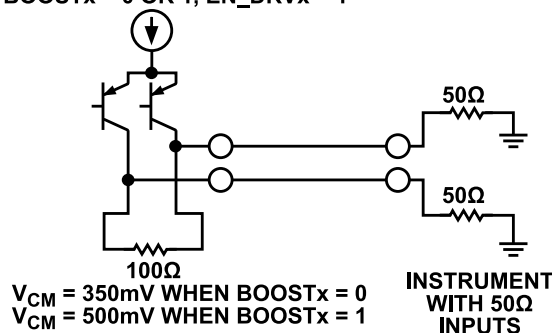
Figure 40. ADF4030 BSYNC Driver to 50 \Omega Instrument Connection
