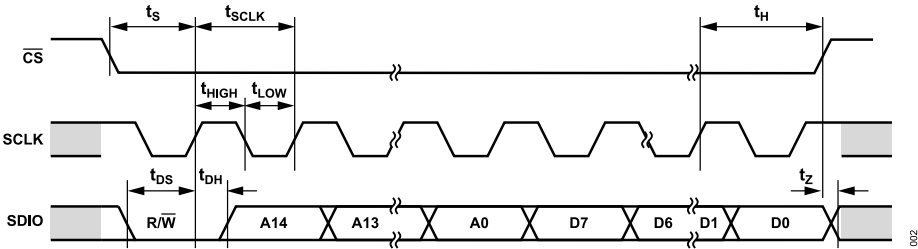
Figure 2. Write Timing Diagram
