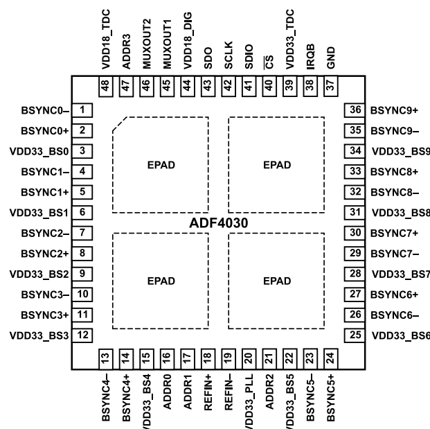
Figure 5. Pin Configuration
