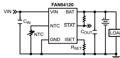
Figure 1. Typical Application
