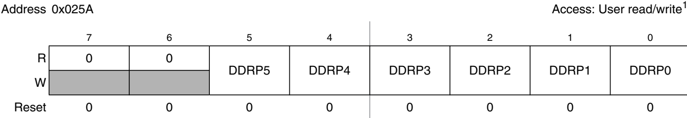
Figure 2-25. Port P Data Direction Register (DDRP)
