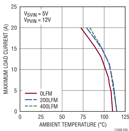
Figure 3. Current Derating at 500kHz, 5V SVIN
