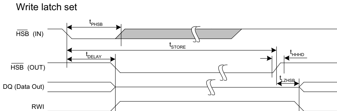
Figure 16. Hardware STORE Cycle [56]
