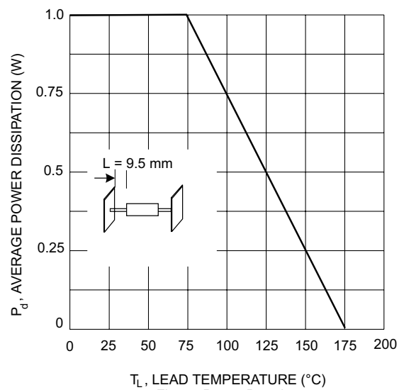
Fig. 5, Power Derating
