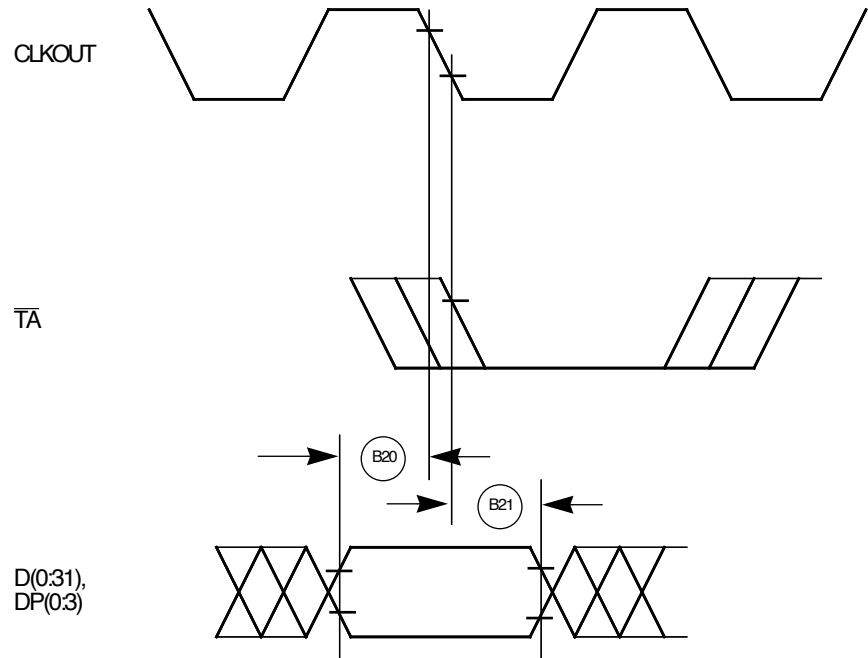
Figure 6. Input Data When Controlled by the UPM Timing Diagram
