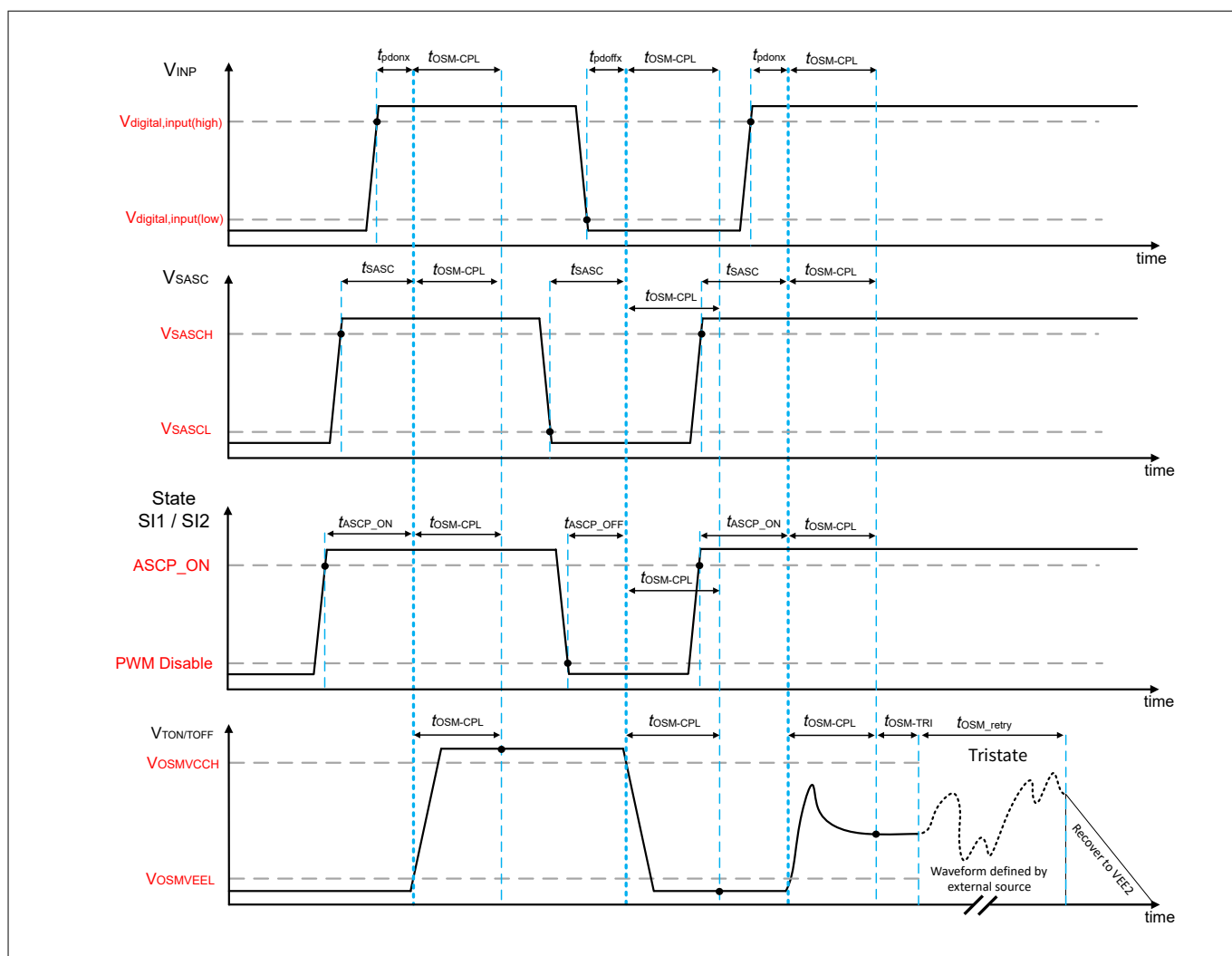
Figure 25 Dynamic output stage monitoring
