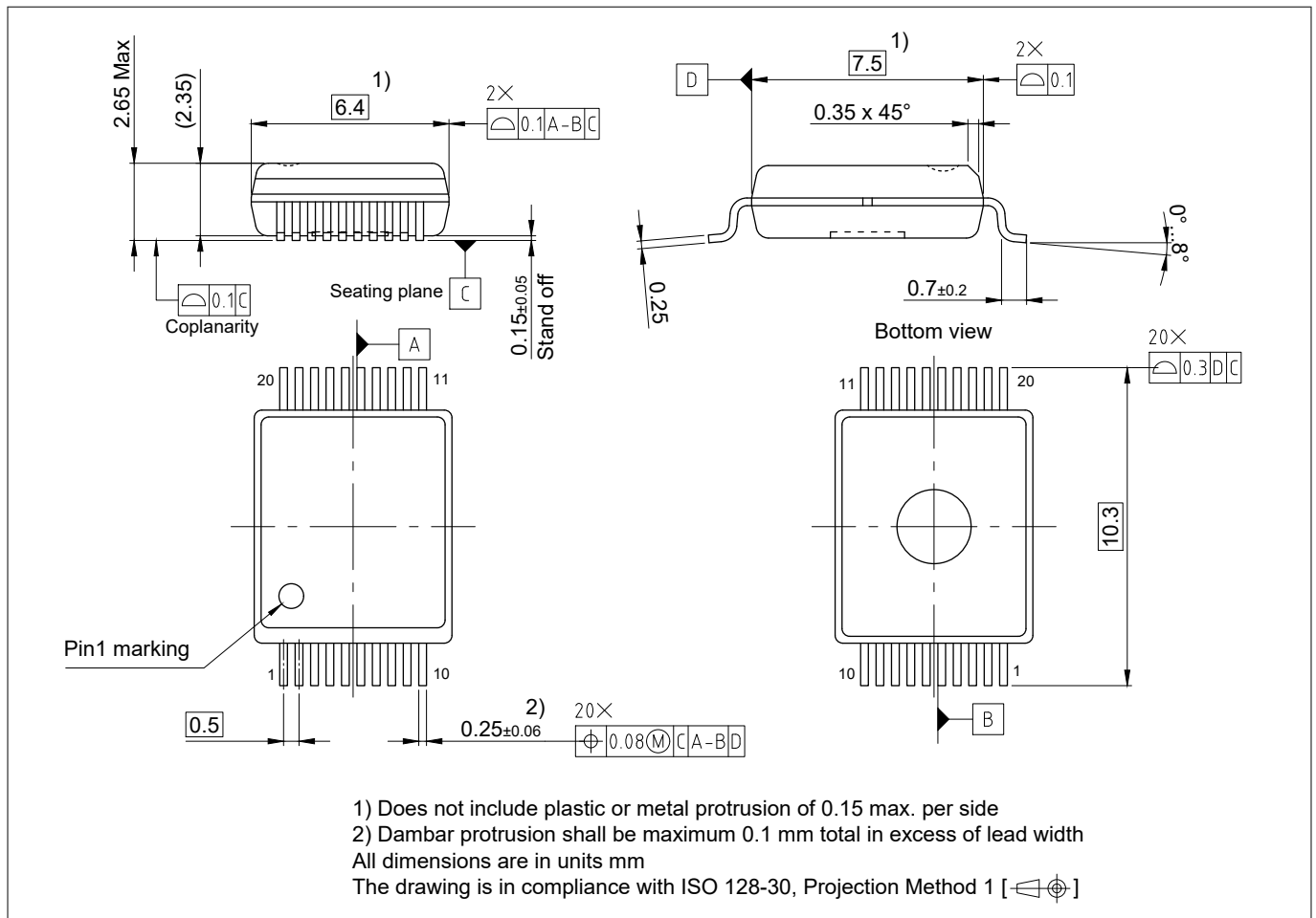
Figure 29 PG-DSO-20
