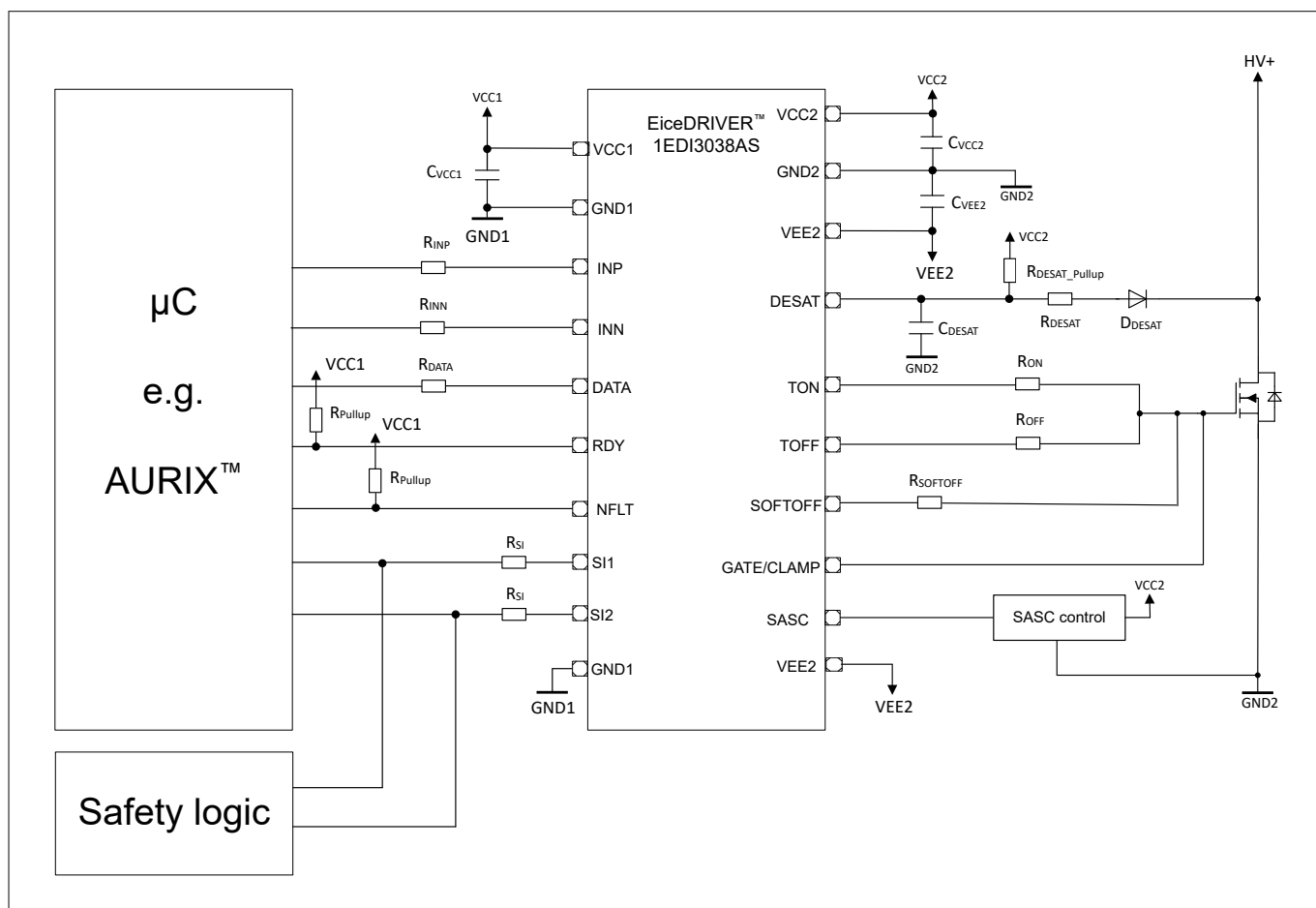
Figure 28 Typical application schematic
