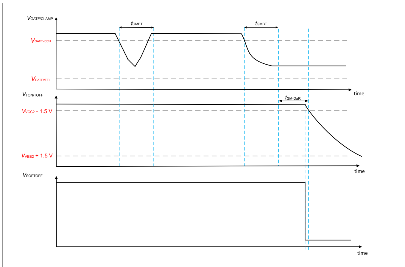
Figure 22 Static gate monitoring timing diagram
