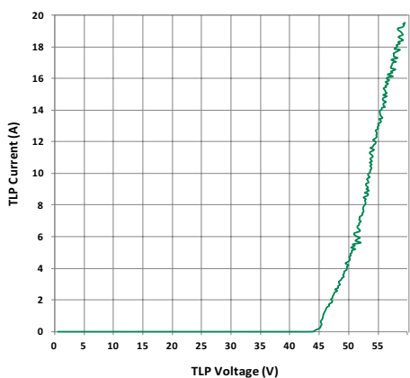
AQ36 Transmission Line Pulsing (TLP) Plot
