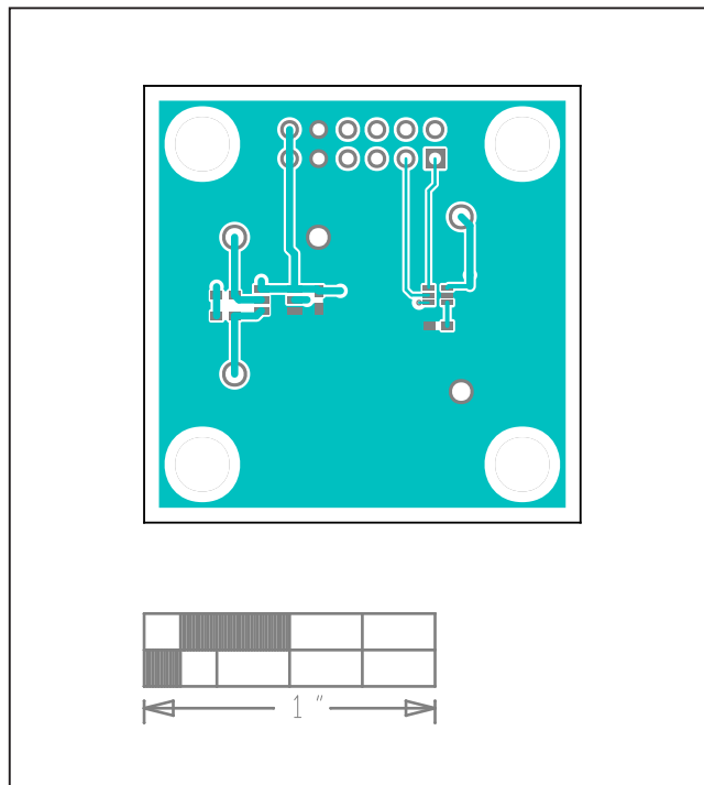
MAX31888 EV Kit-Top
