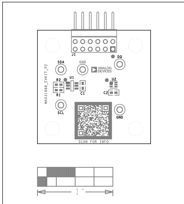
MAX31888 EV Kit-Silk Top
