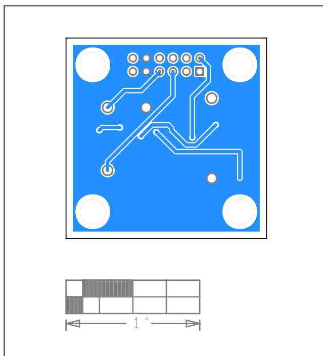
MAX31888 EV Kit-Bottom
