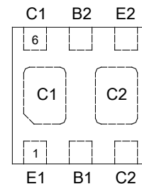
Top View Pinout
