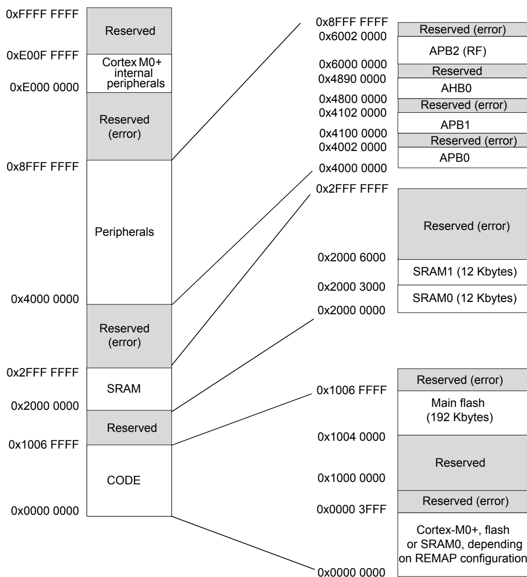
Figure 9. Memory map
