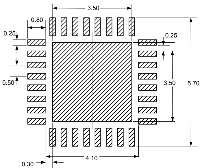
Figure 19. VFQFPN32 - Footprint example
