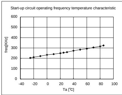
Fig.1 Start-up circuit frequency-Temp
