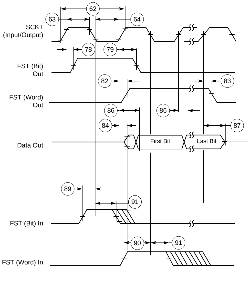
Figure 36. ESI Transmitter Timing
