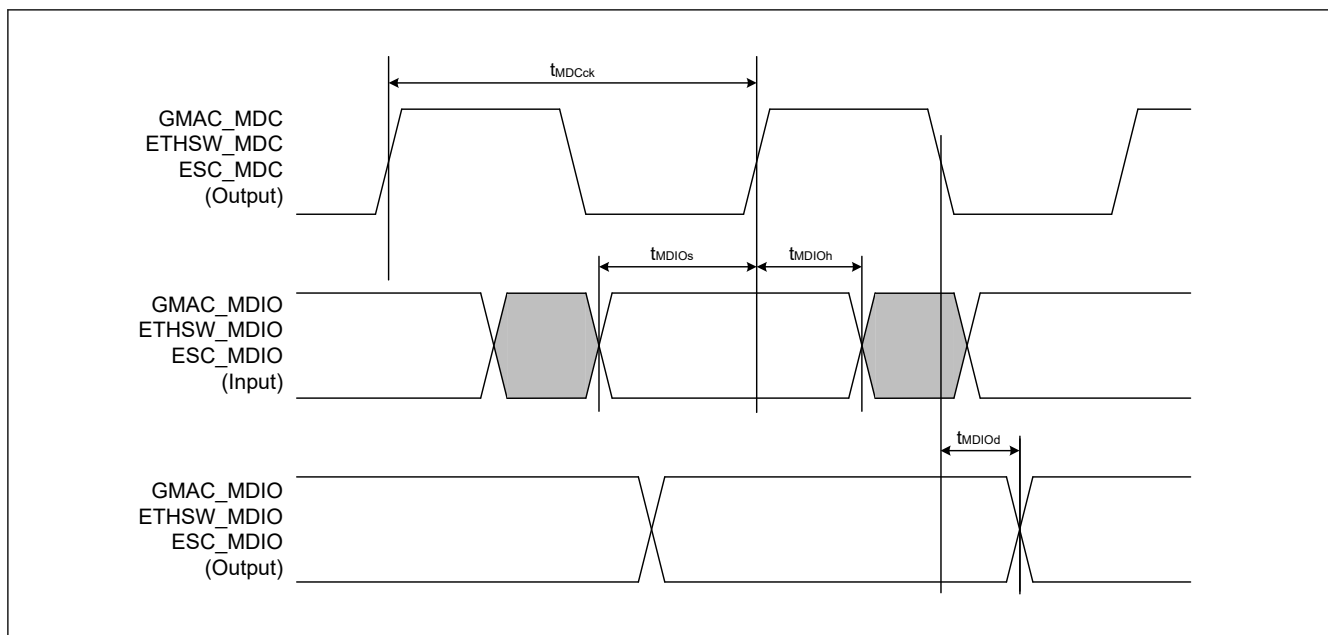
Figure 2.88 Serial management interface timing
