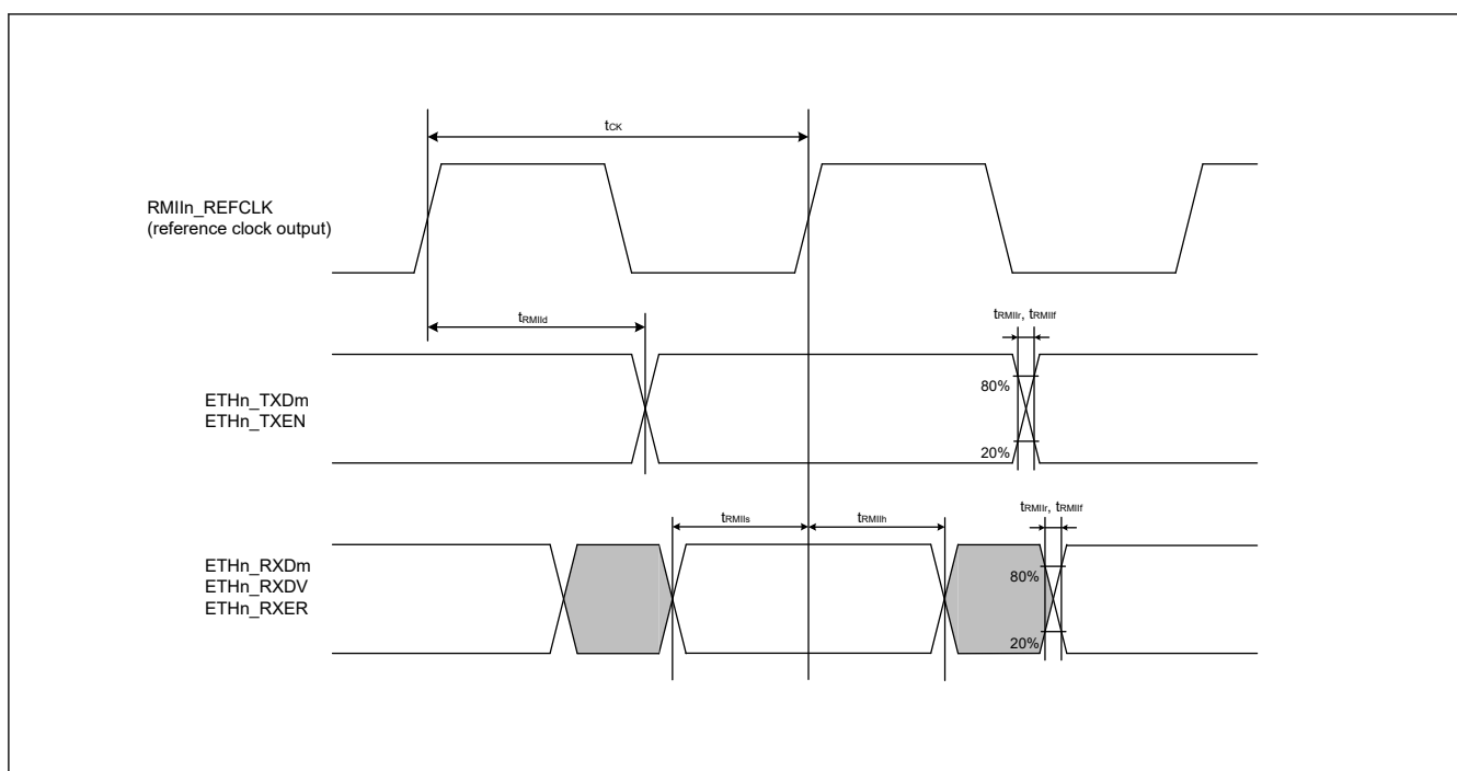
Figure 2.83 RMII transmission and reception timing (reference clock output) ( n = 0 to 2, m = 0 to 1)
