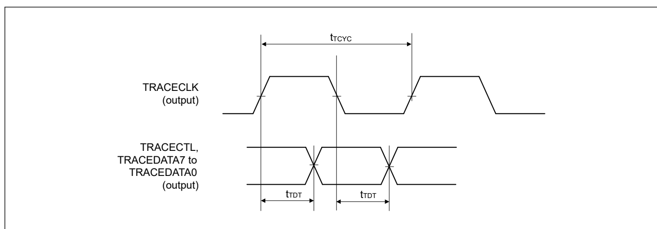
Figure 2.99 Trace interface timing
