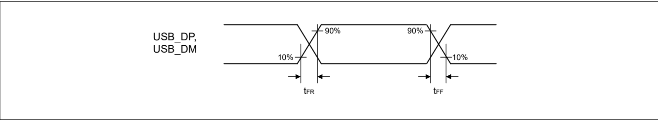
Figure 2.91 USB_DP, USB_DM output timing (full speed)
