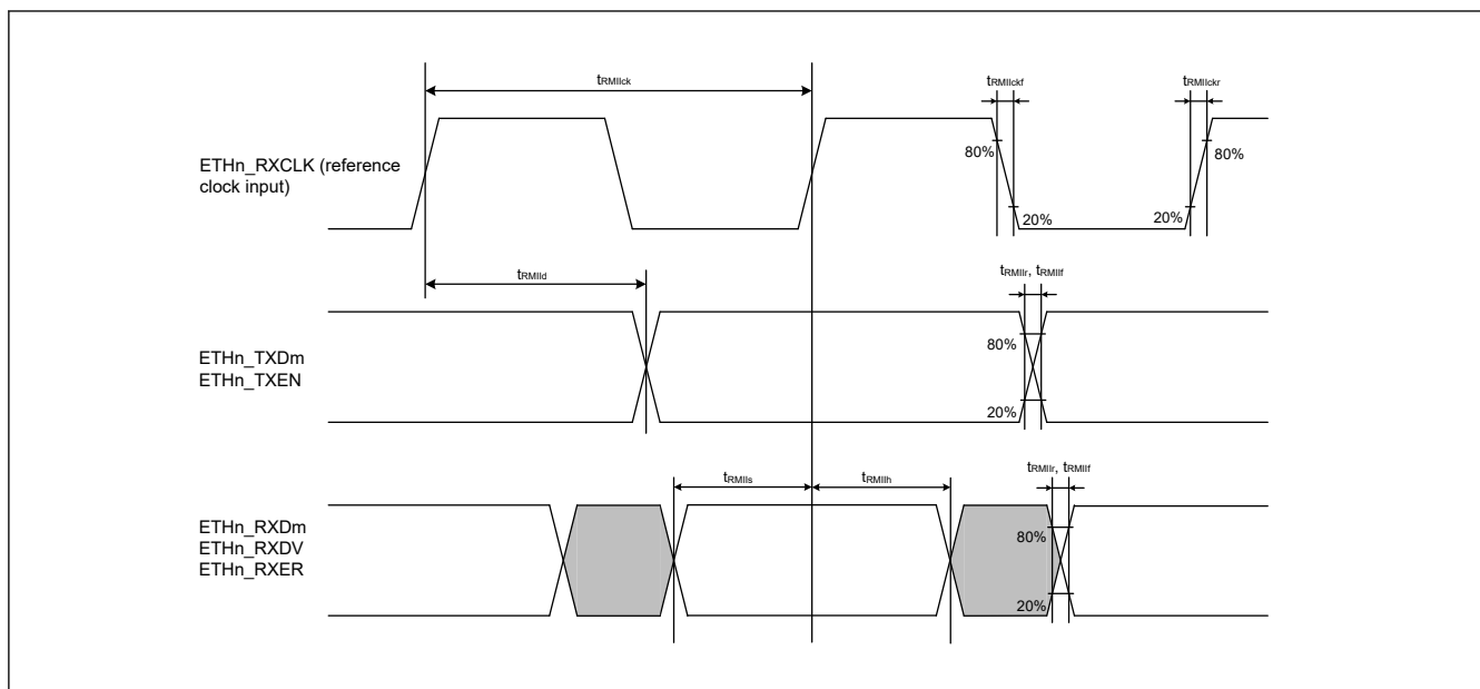
Figure 2.82 RMII transmission and reception timing (reference clock input) ( n = 0 to 2, m = 0 to 1)
