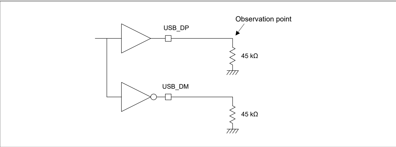
Figure 2.94 Measurement circuit (high speed)
