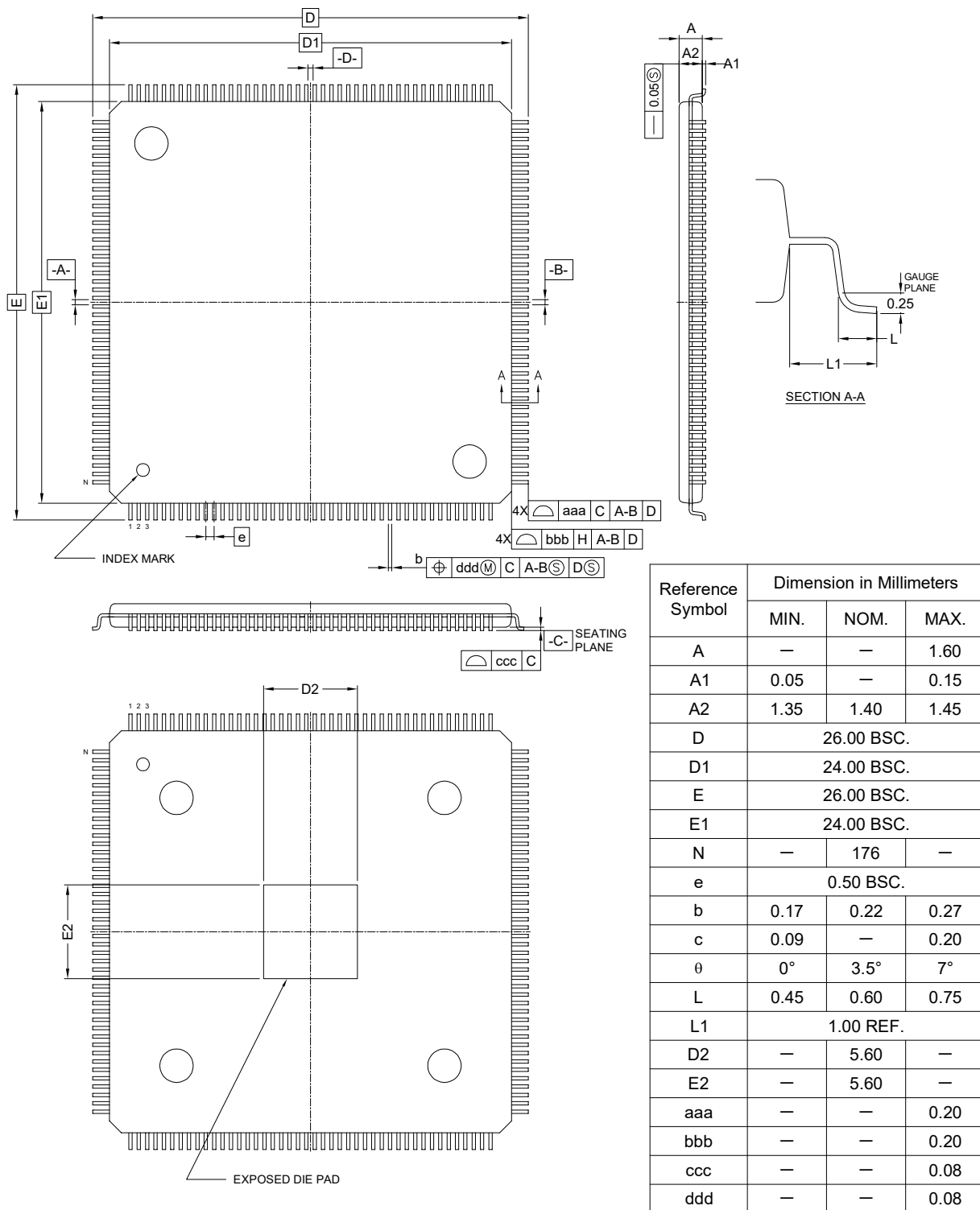
Figure A1.3 176-pin LQFP with exposed die pad
