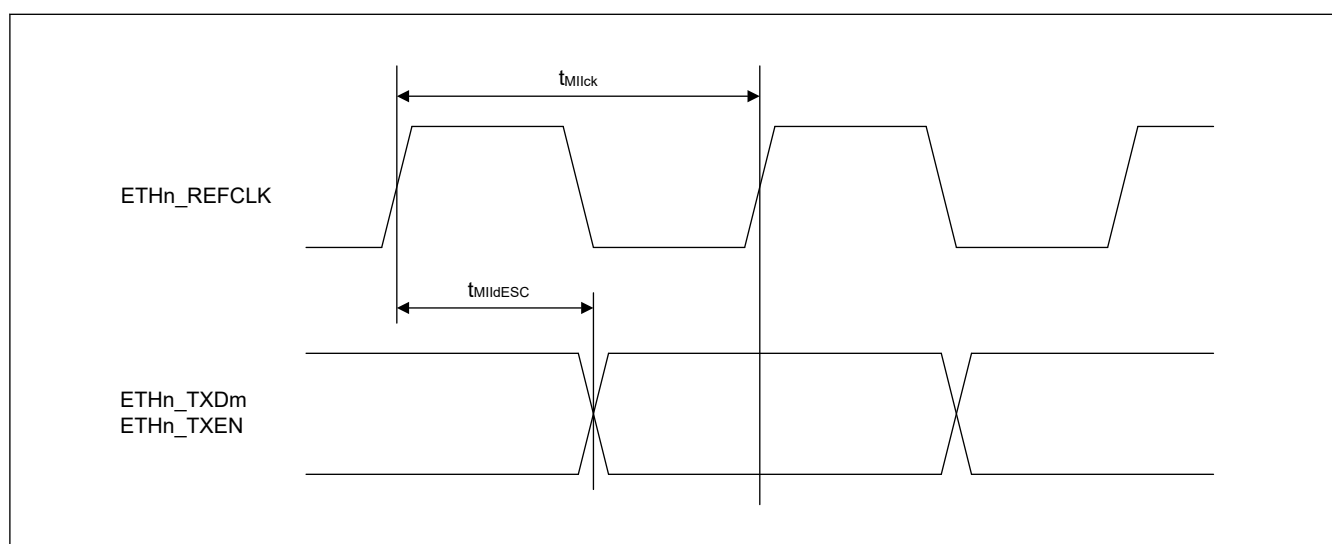
Figure 2.85 ESC MII transmission timing (automatic TX shift disabled) ( n = 0 to 2 , m = 0 to 3 )
