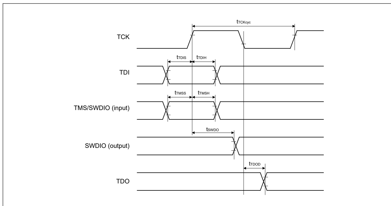
Figure 2.97 Data transfer timing
