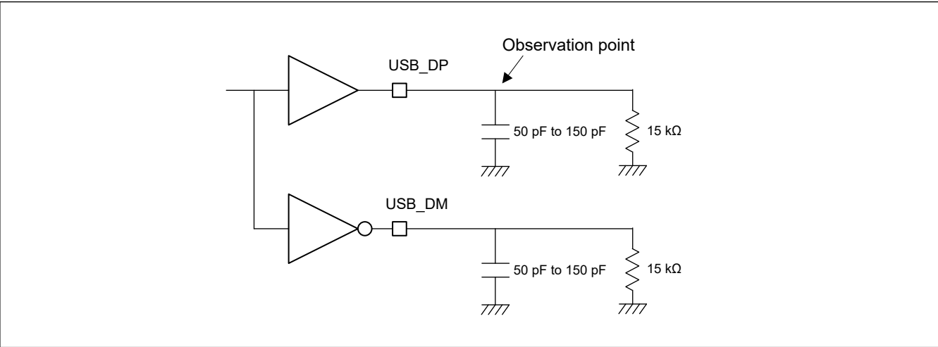
Figure 2.90 Measurement circuit (low-speed/host only)
