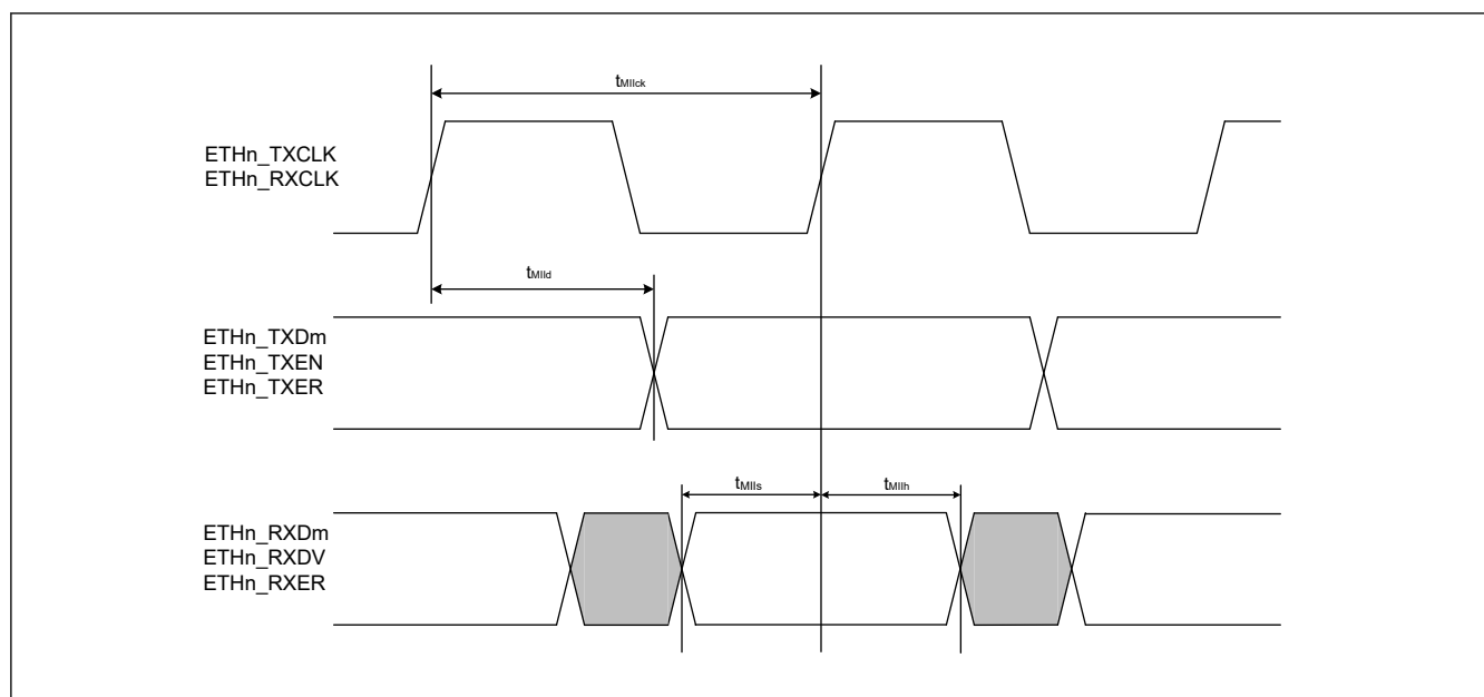
Figure 2.84 MII transmission and reception timing ( n = 0 to 2 , m = 0 to 3 )
