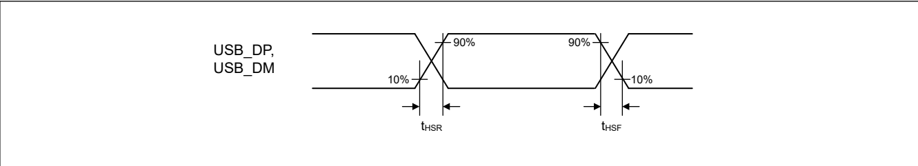
Figure 2.93 USB_DP, USB_DM output timing (high speed)
