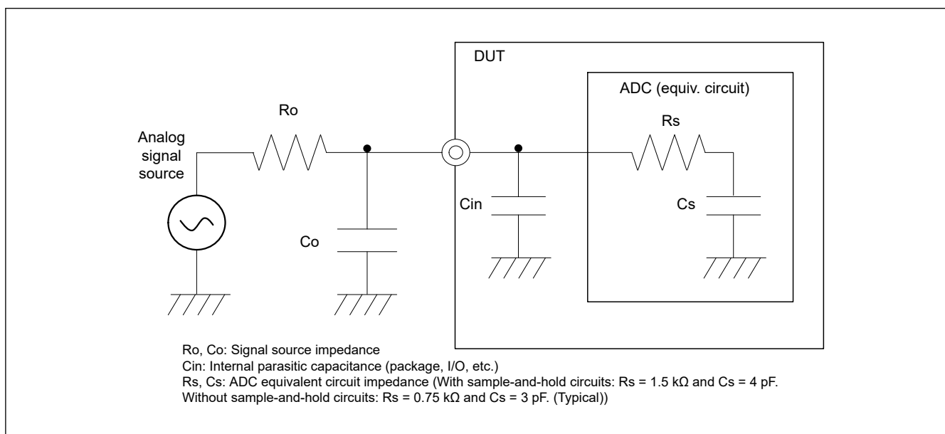
Figure 2.95 A/D converter equivalent circuit and peripheral configuration diagram
