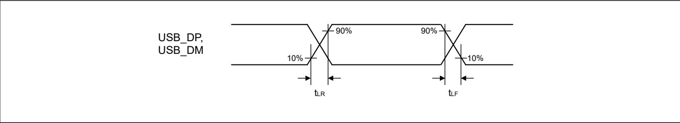
Figure 2.89 USB_DP, USB_DM output timing (low-speed/host only)
