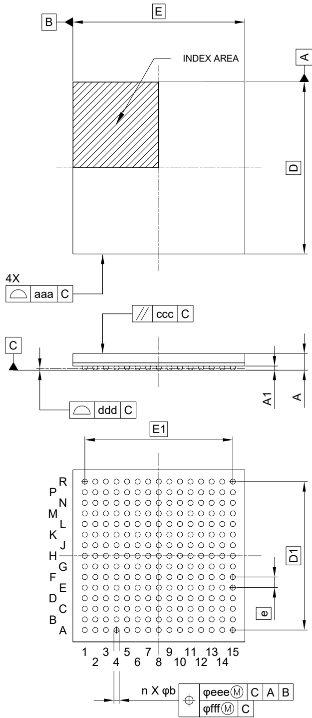
Figure A1.2 225-pin FBGA
