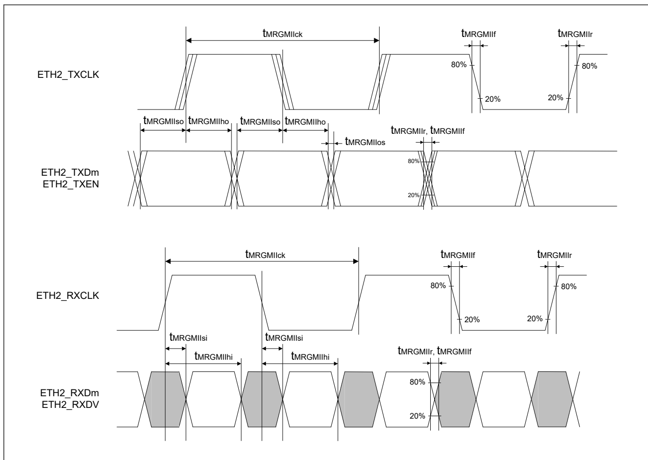
Figure 2.86 RGMII transmission and reception timing (MAC to MAC connection mode) (m = 0 to 3)
