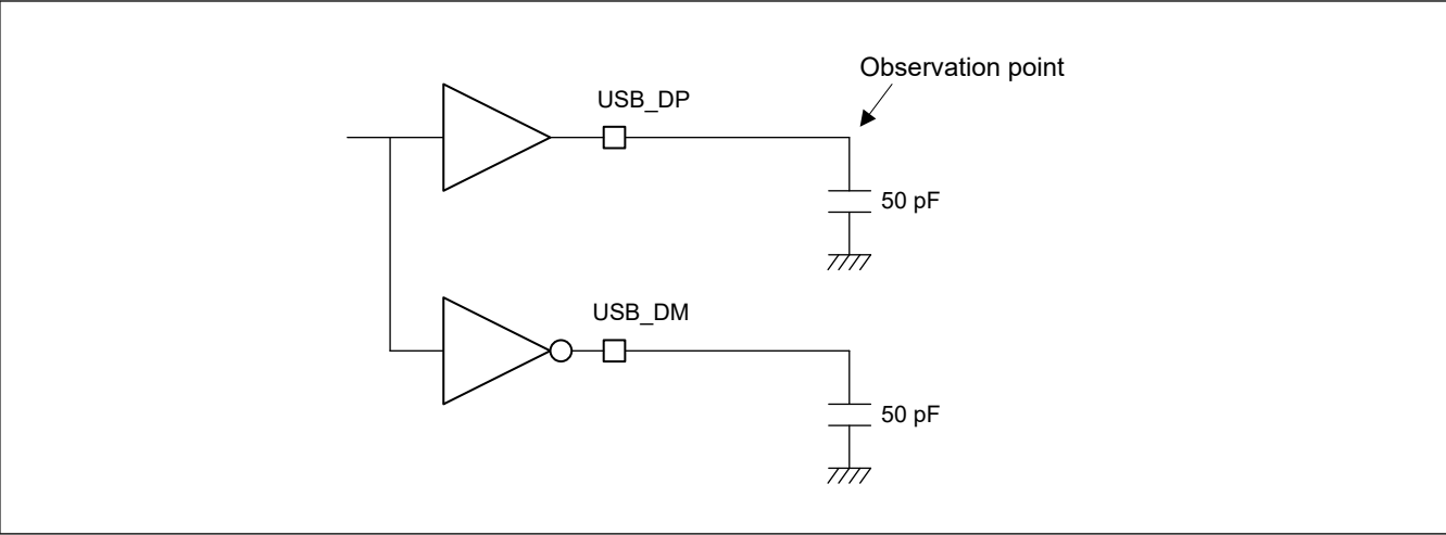
Figure 2.92 Measurement circuit (full speed)
