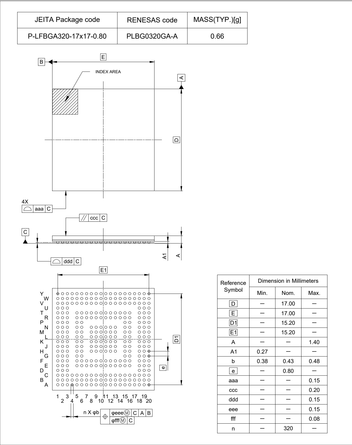
Figure A1.1 320-pin FBGA
