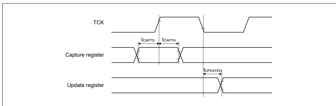
Figure 2.98 Boundary scan input/output timing
