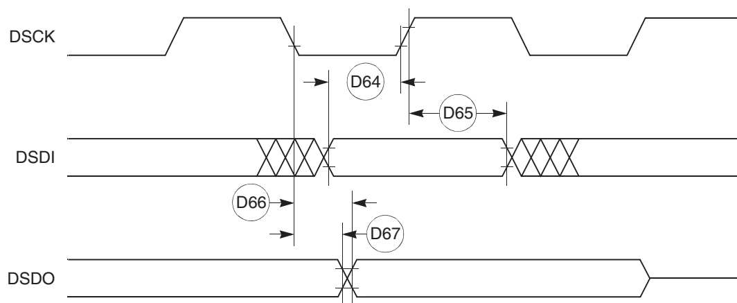
Figure 8-29. Debug Port Timings
