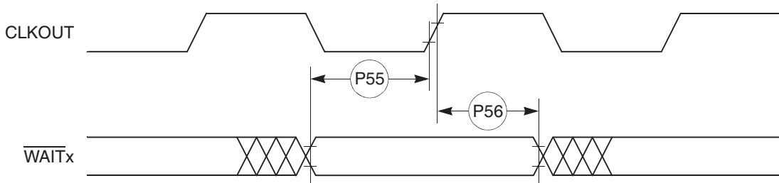
Figure 8-25. PCMCIA \overline{WAIT} Signals Detection Timing
