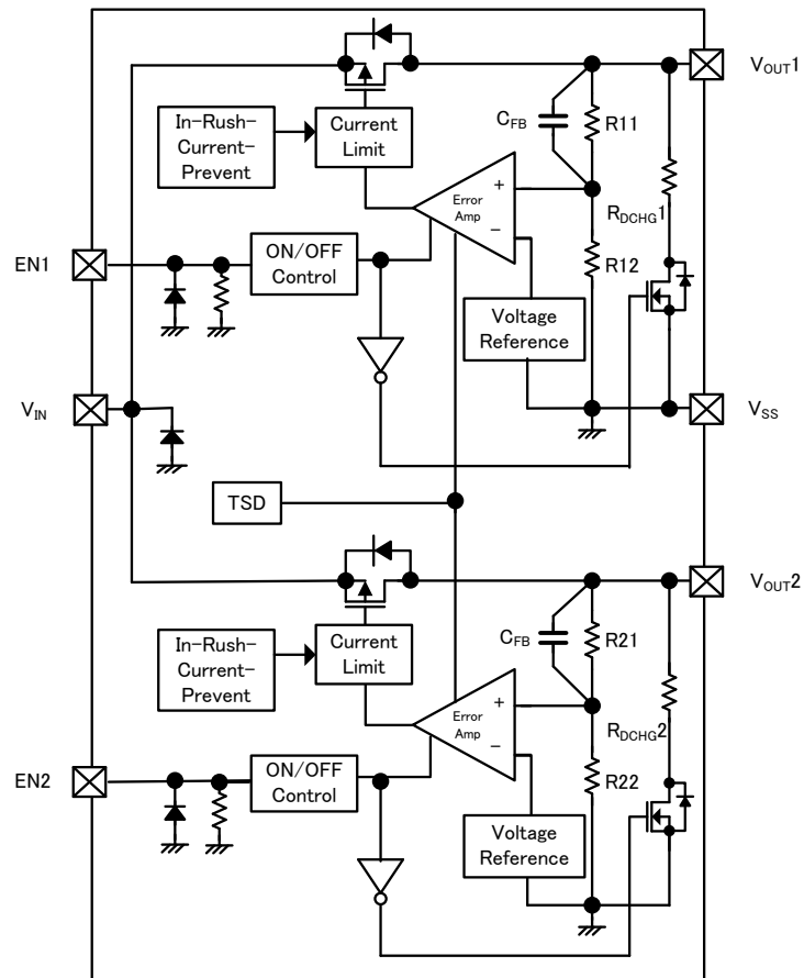
XC6421ABxxxseries
