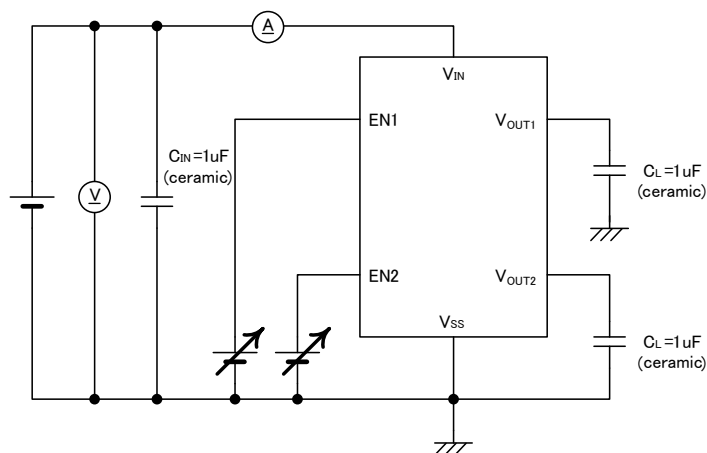
● Circuit ②
