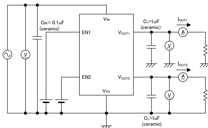
● Circuit ③
