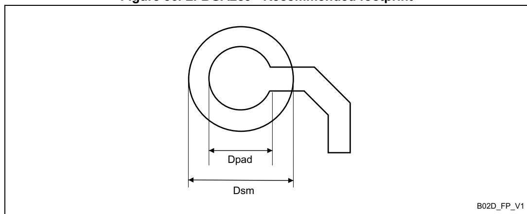
Figure 56. LFBGA289 - Recommended footprint
