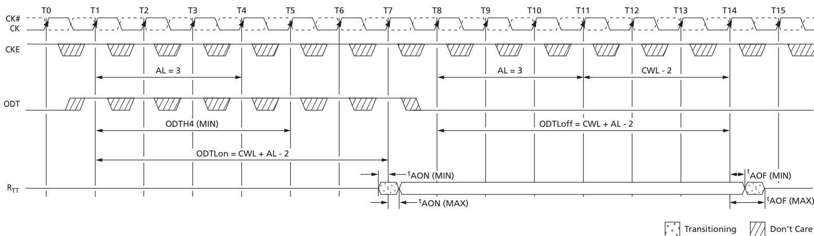
Figure 113: Synchronous ODT
