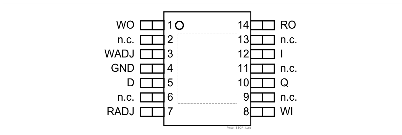
Figure 2 Pin Assignment PG-SSOP14 Package
