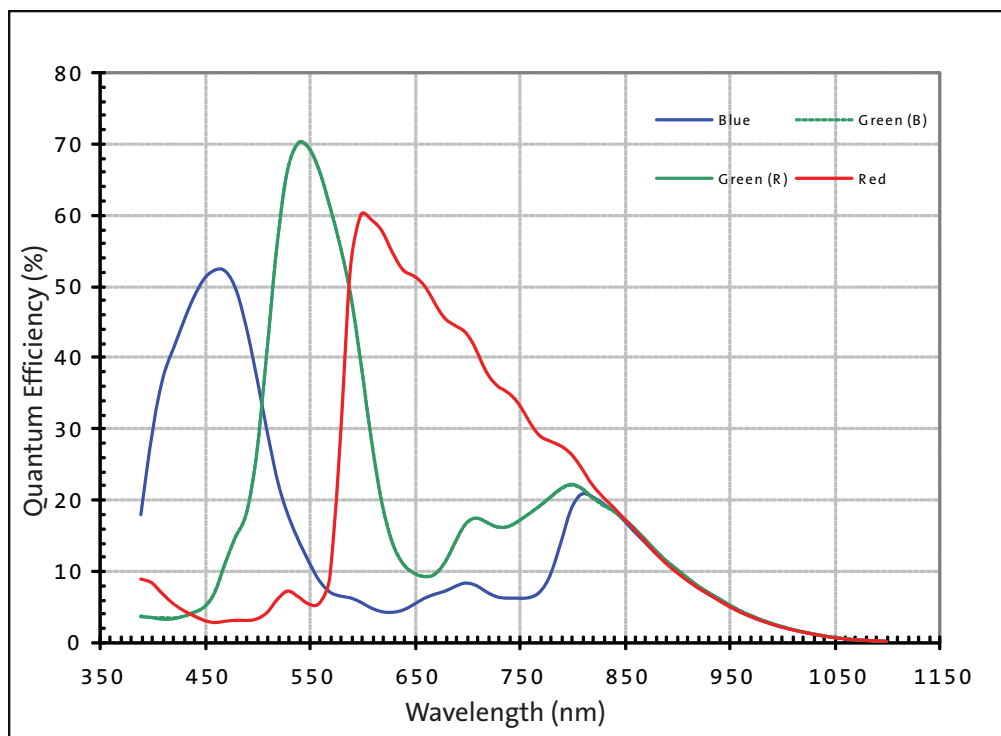
Figure 60: Quantum Efficiency
